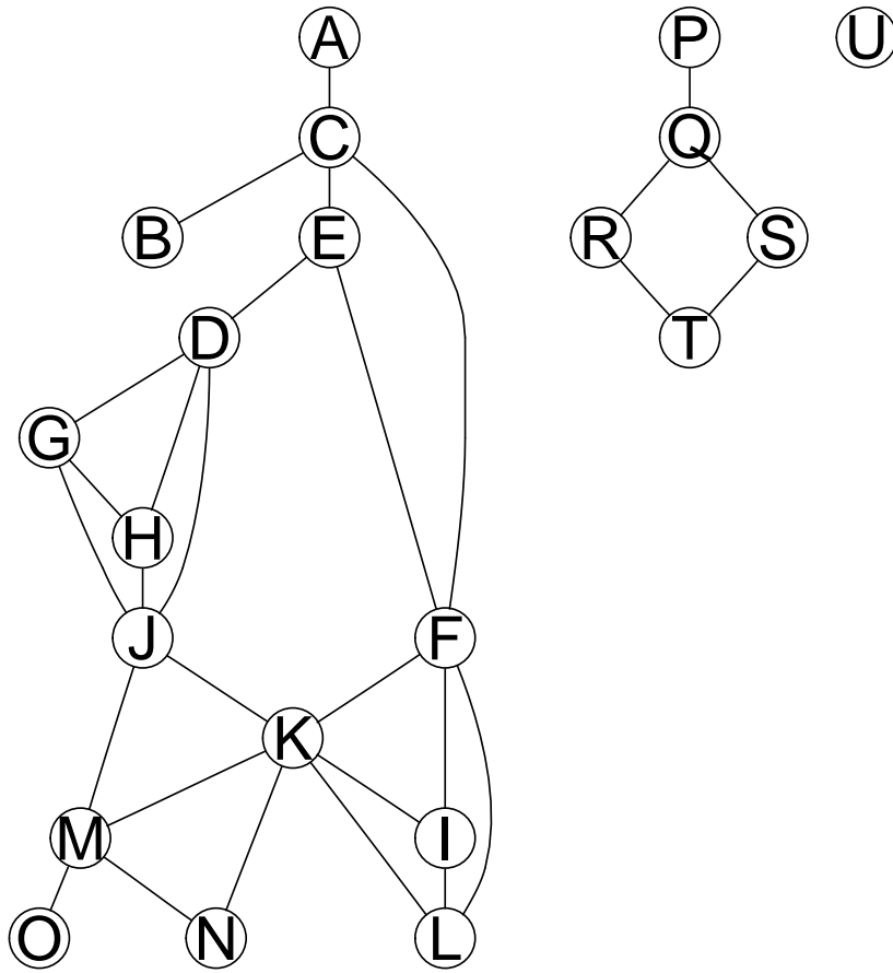
Figure 15: K-cores Example.
