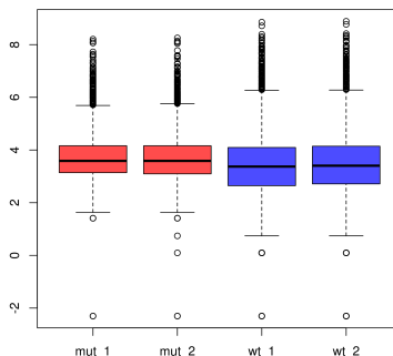
Figure 4: Between-lane distribution of gene-level counts (log).
