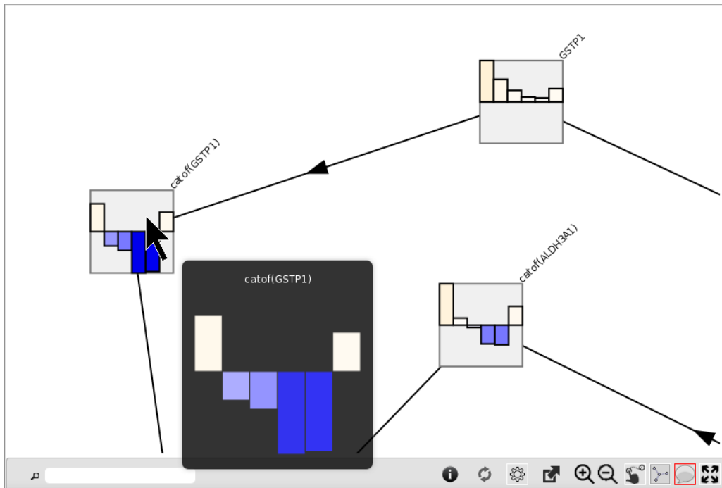
Figure 22: Tooltips
