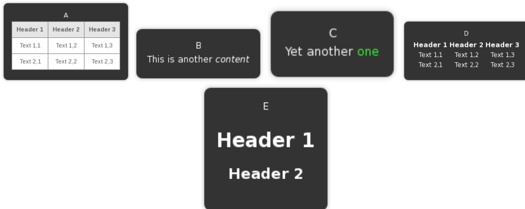
Figure 11: Custom Tooltips
