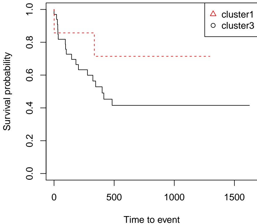
Kaplan–Meier curve
