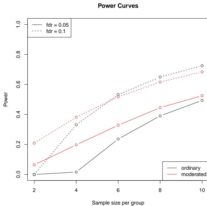
Figure 7: Estimated average power for other sample sizes than that of the pilot-data for both moderated and original t test-statistics and for different false discovery rate thresholds.
